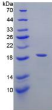
Figure 2. SDS-PAGE
