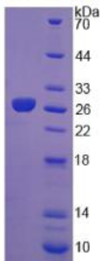
Figure 1. SDS-PAGE
