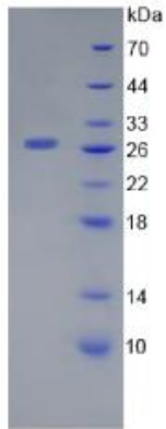
Figure 1. SDS-PAGE
