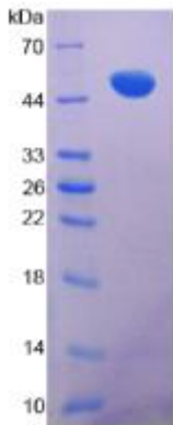
Figure 1. SDS-PAGE
