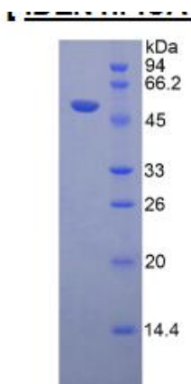
Figure 1. SDS-PAGE
