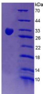
Figure 1. SDS-PAGE
