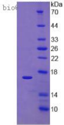
Figure 2. SDS-PAGE
